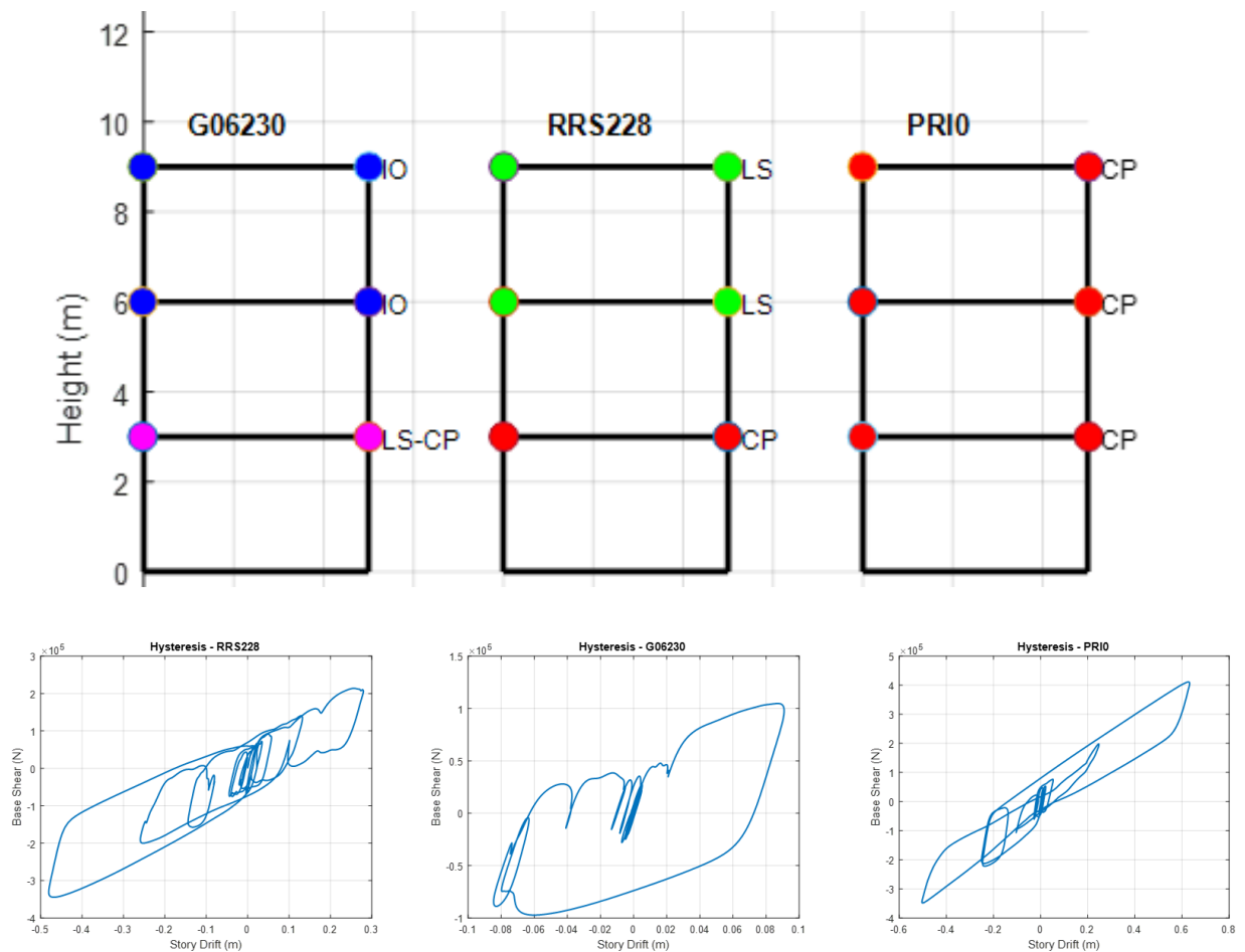
Figure 4. Damage states and corresponding hysteretic curves under near-fault pulse-like earthquakes
