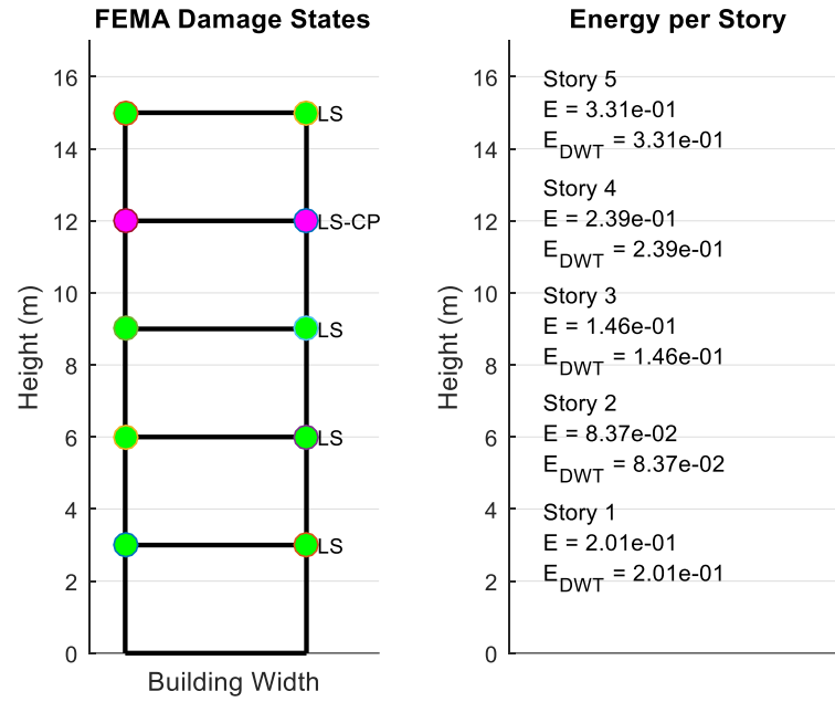
Figure 4. Damage states and corresponding energies under near-fault pulse-like earthquakes
