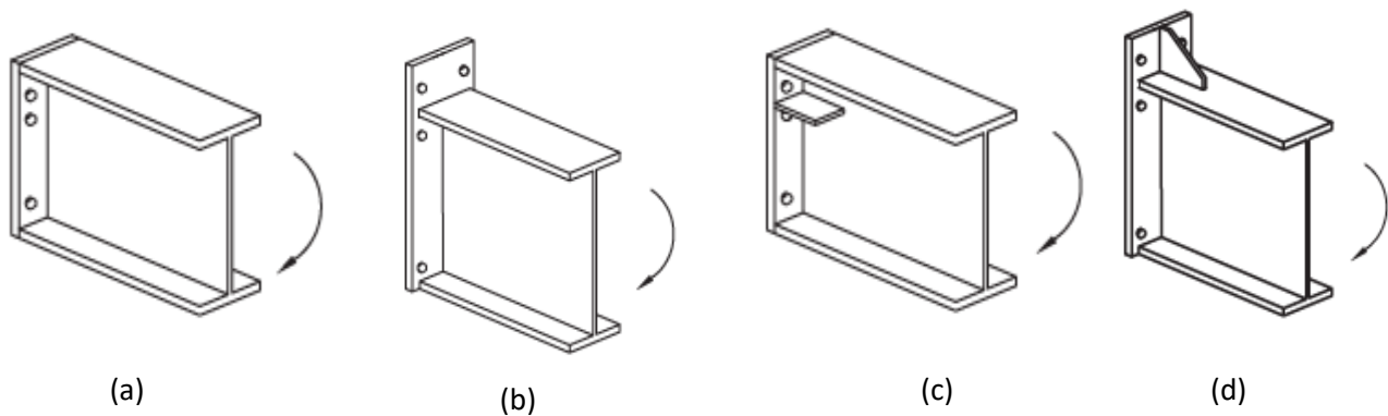
Figure 2 Flush (a), Extend (b,) Stiffened Flush (c) and Stiffened Extended (d) End-plate Moment Connections
