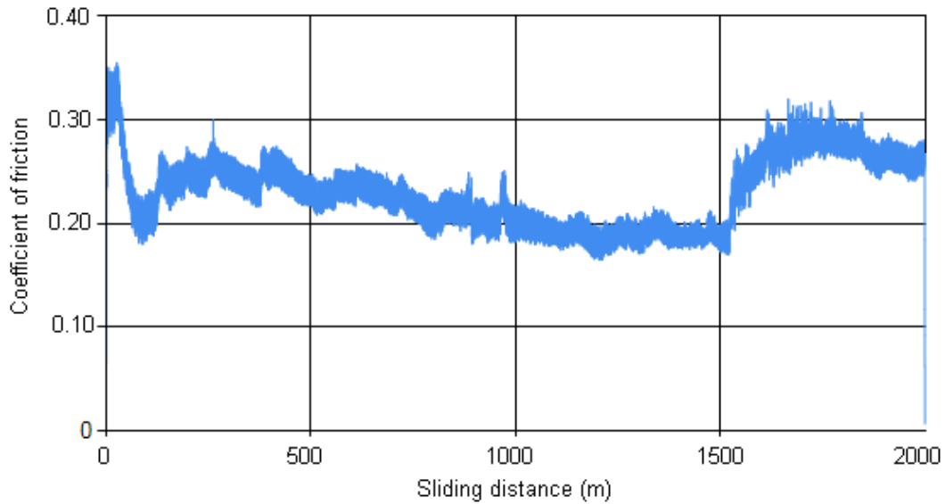
Figure 1. The COF versus sliding distance for a PA66/30CF composite operating at the speed of 1.0 m/s and under the load of 100 N
