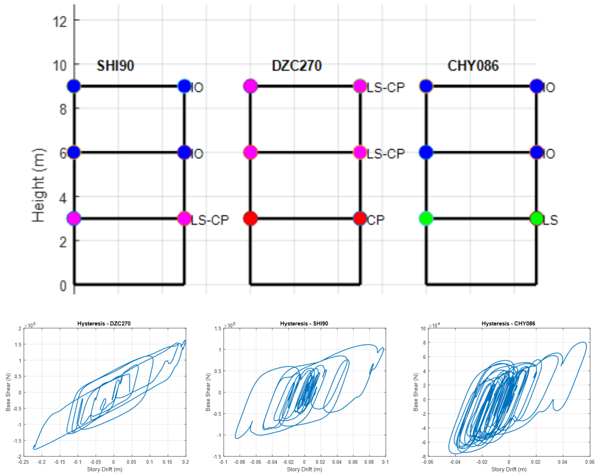
Figure 2. Damage states and corresponding hysteretic curves under far-fault earthquakes
