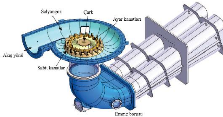
Figure 4. Francis Tipi Türbin [17]
