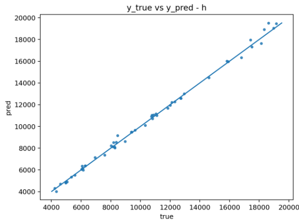
Figure 2. Parity plot for the most challenging PINN target ( h , heat-transfer coefficient).
