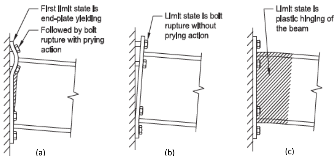
Figure 3 The Thin (a), The Thick (b) End Plate Thickness and The Strong Column & Weak Beam (c)
