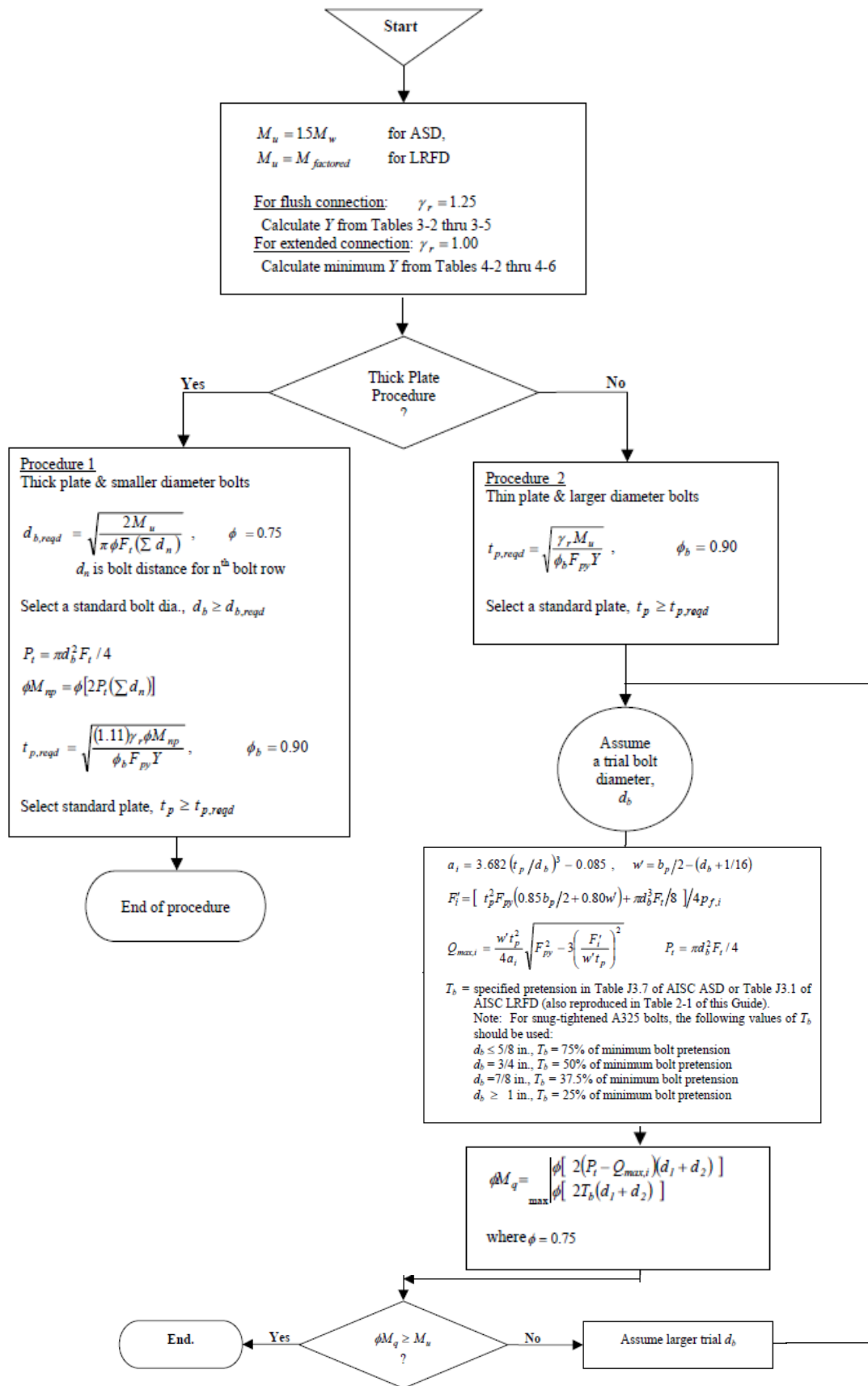
Figure 4 Flow Chart for General Design Procedure for End-Plate Connections
