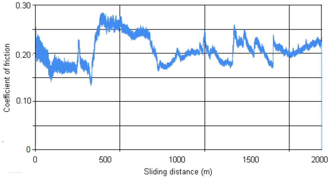
Figure 3. The COF versus sliding distance for a PA66/30CF composite operating at the speed of 3.0 m/s and under the load of 100 N
