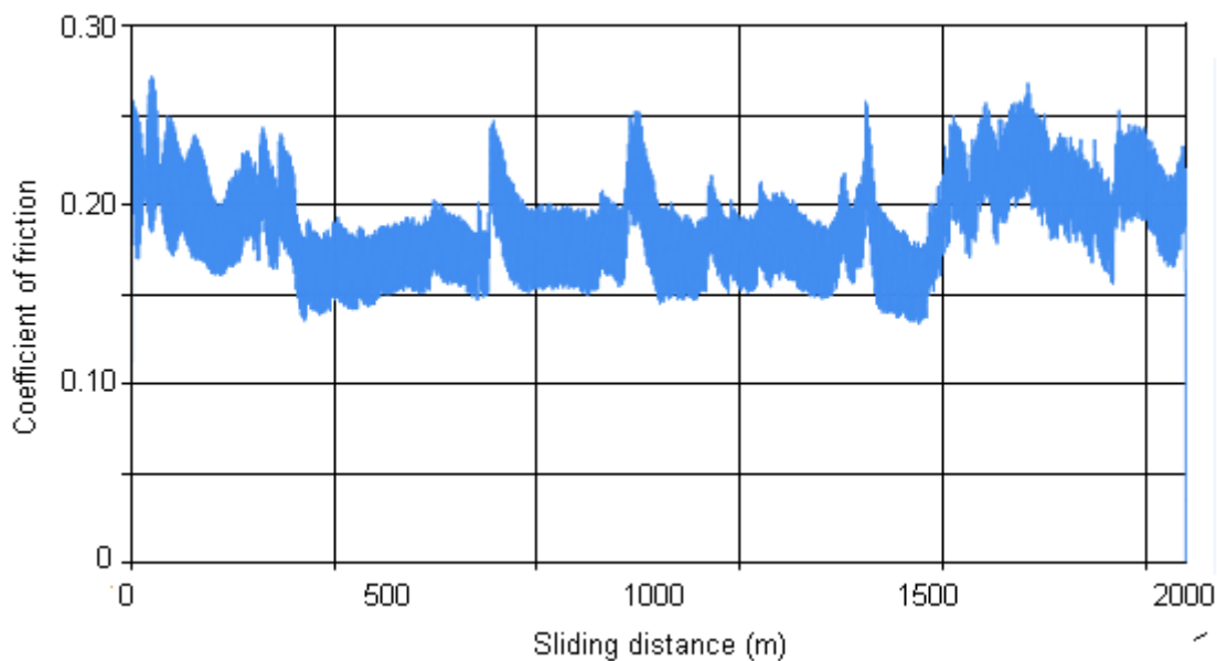
Figure 2. The COF versus sliding distance for a PA66/30CF composite operating at the speed of 2.0 m/s and under the load of 100 N
