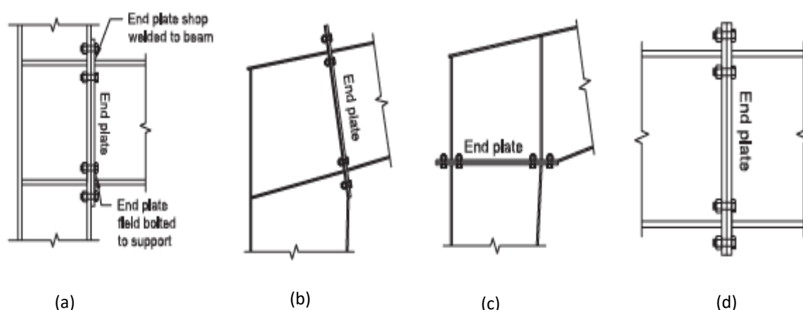
Figure 1 Vertical Connection (a), Inclined Connection (b), Horizontal Connection (c), Splice Connection (d)
