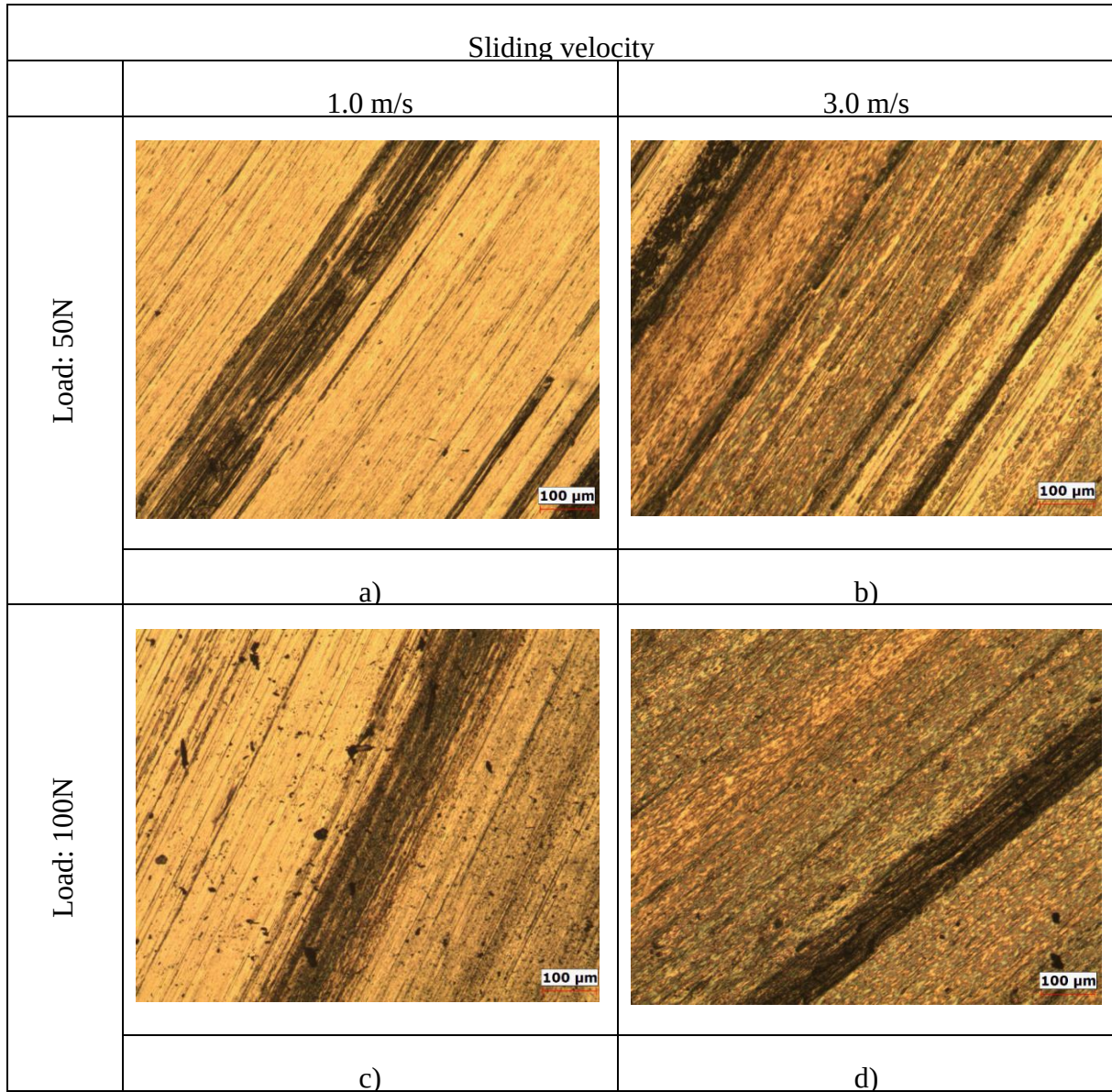
Figure 5. Optical microscope images taken from the wear surface of a steel disc under different loads (50 and 100 N) and at different speeds (1.0 and 3.0 m/s)
