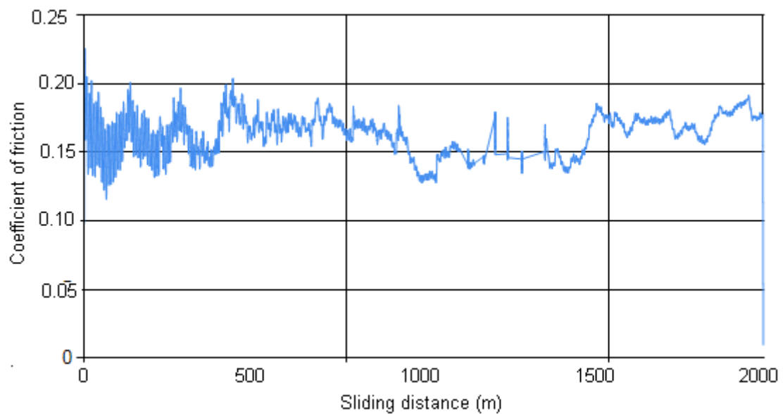
Figure 4. The COF versus sliding distance for a PA66/30CF composite operating at the speed of 4.0 m/s and under the load of 100 N
