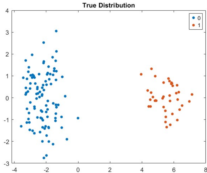
Figure 2. PCA Visualization of the true distribution of the normal and anomalous sequences.
