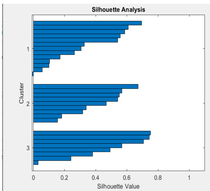
Figure 4. Silhouette analysis for each cluster
