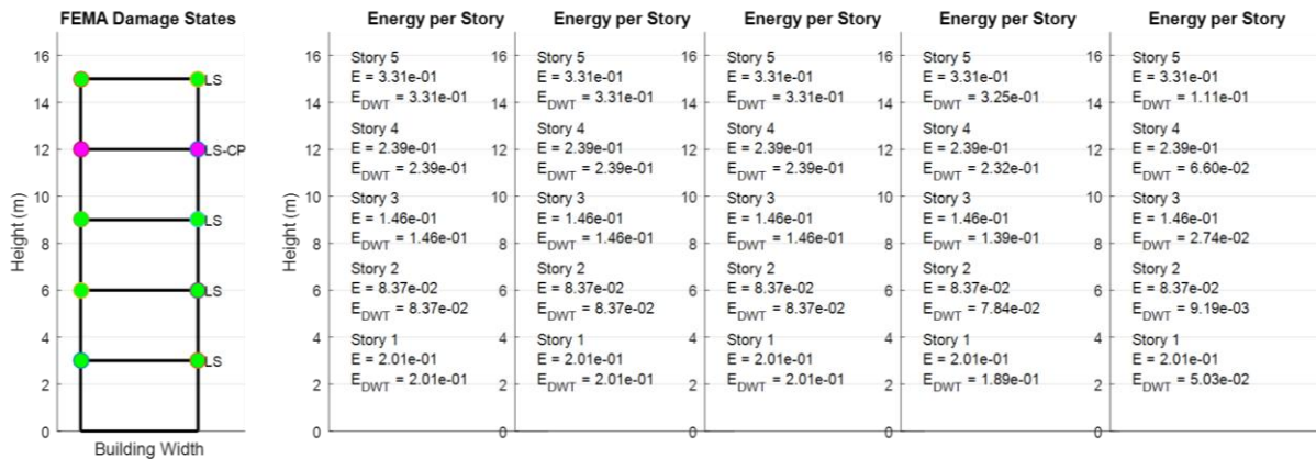
Figure 5. Damage states and energies for different level decompositions
