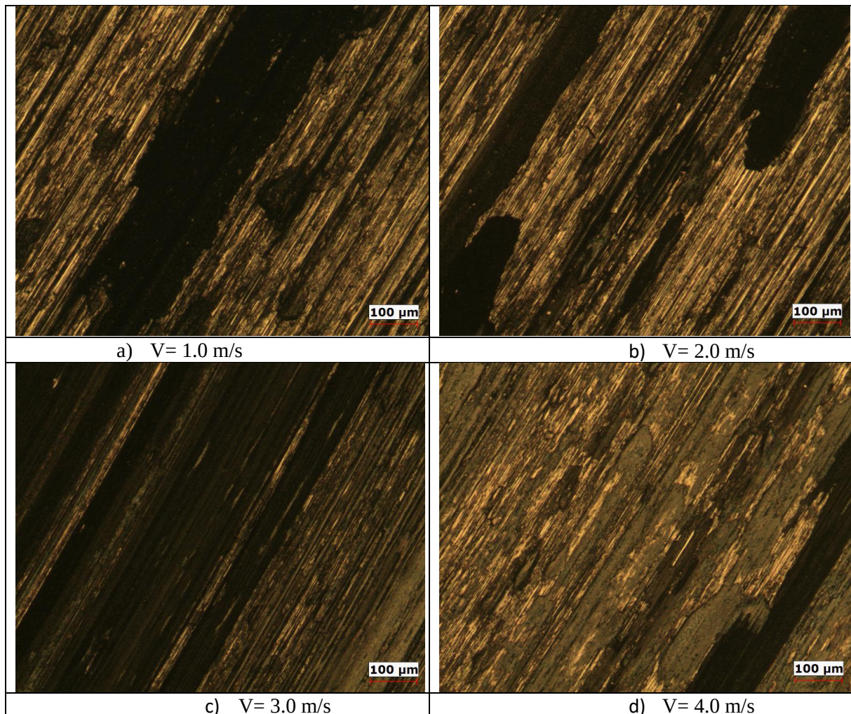
Figure 9. Optical microscope images of the wear surfaces of stainless steel discs in contact with PA66/30CF composites at different speeds: a) 1.0 m/s, b) 2.0 m/s, c) 3.0 m/s and d) 4.0 m/s
