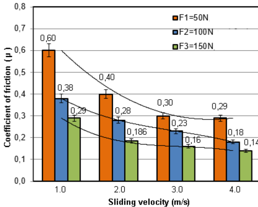
Figure 3. Variation in the CoF of the POM/25GF composite as a function of velocity under different loads
