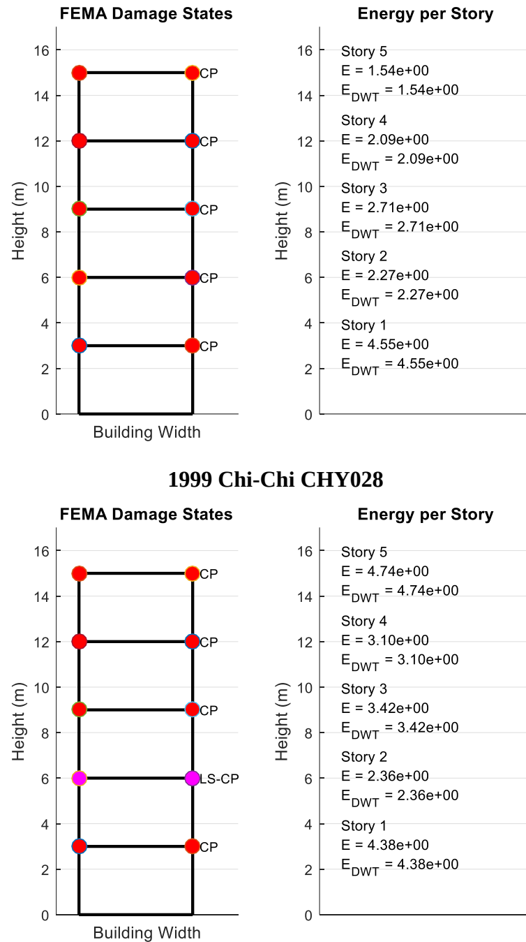
Figure 3. Damage states and corresponding energies under near-fault no-pulse earthquakes
