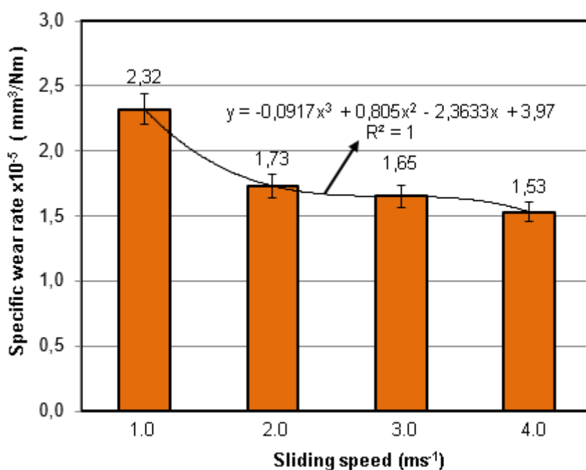
Figure 6. Variation in the SWR of the PA66/30CF composite as a function of sliding speed
