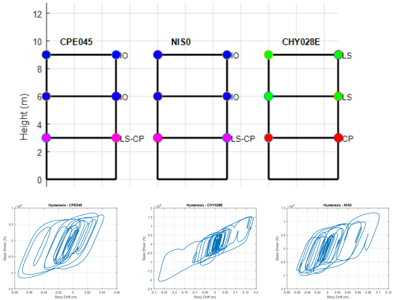
Figure 3. Damage states and corresponding hysteretic curves under near-fault no-pulse earthquakes
