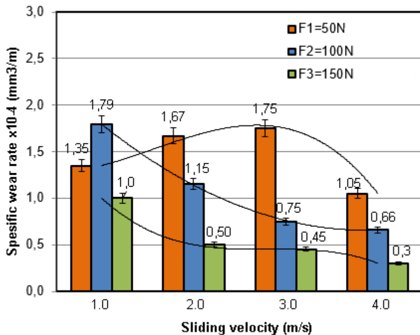
Figure 4. Variation in the s-WR of the POM/25GF composite as a function of velocity under different loads
