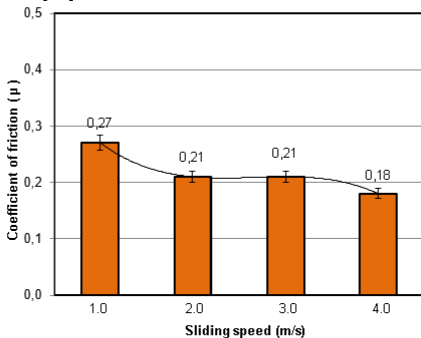
Figure 5. Variation in the COF of PA66/30CF composite as a function of sliding speed
