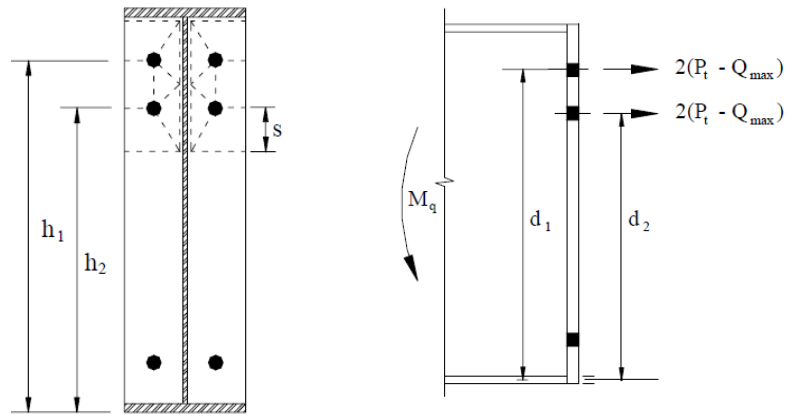
Figure 15 Four-Bolt Flush Unstiffened Moment End-Plate
