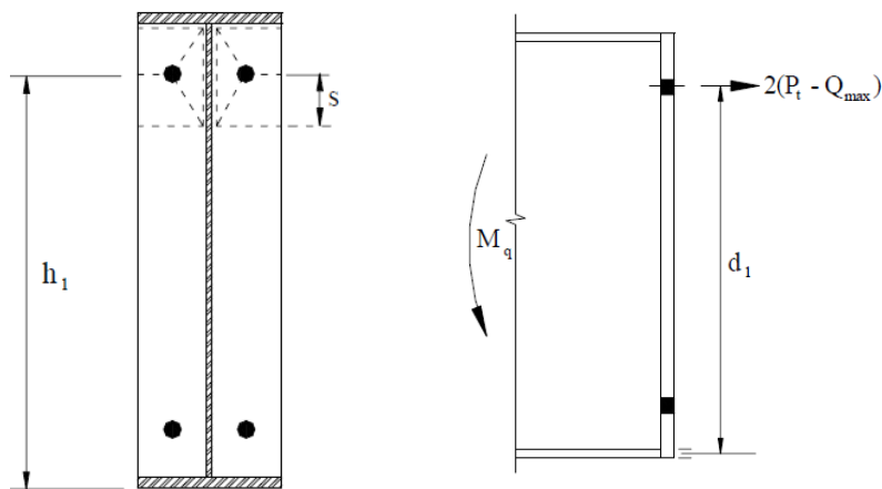
Figure 14 Two-Bolt Flush Unstiffened Moment End-Plate
