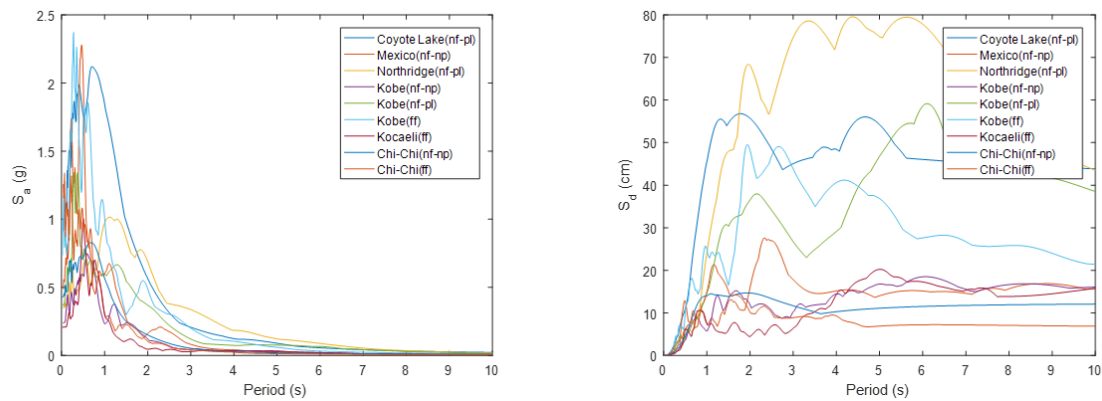
Figure 1. Acceleration and displacement spectra
