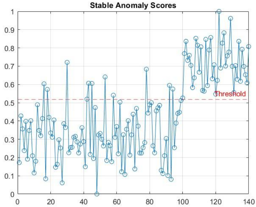
Figure 1. Anomaly score distribution
