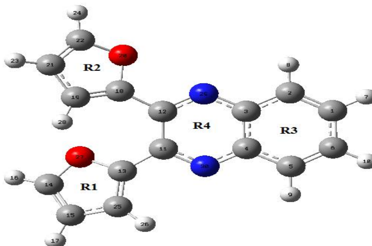
Figure1. The Stable Structure of The 2,3-difurylquinoxaline
