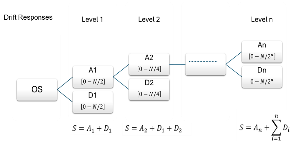
Figure 1. Schematic of DWT applied to drift responses
