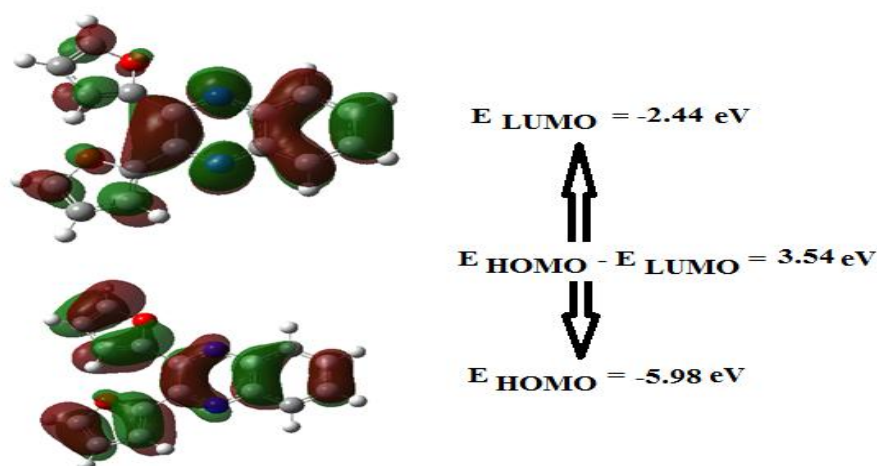
Figure 2. HOMO-LUMO Molecular Orbitals of The 2,3-difurylquinoxaline
