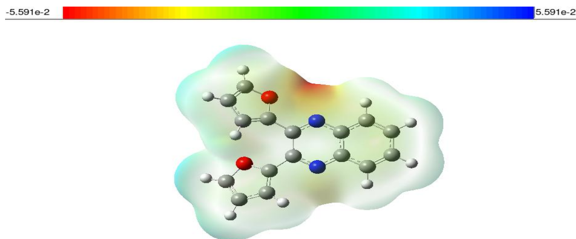
Figure 3. Molecular Electrostatic Potential Surface Map (MEP) of The 2,3-difurylquinoxaline
