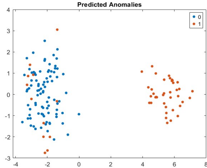
Figure 3. PCA Visualization of the predicted anomaly labels
