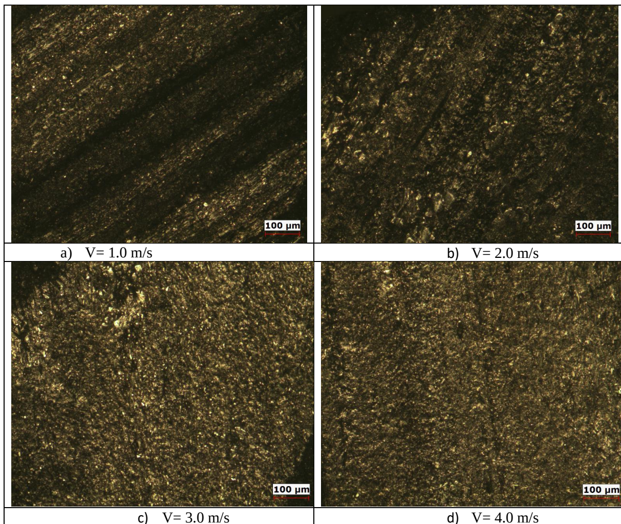
Figure 8. Optical microscope images of the wear surface of a PA66/30CF composite pin at different speeds: a) 1.0 m/s, b) 2.0 m/s, c) 3.0 m/s and d) 4.0 m/s
