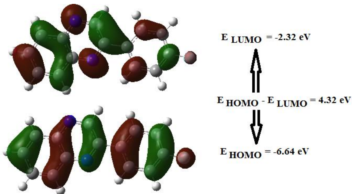
Figure 2. HOMO-LUMO Molecular Orbitals of the 2-(4-Fluorophenyl)quinoxaline
