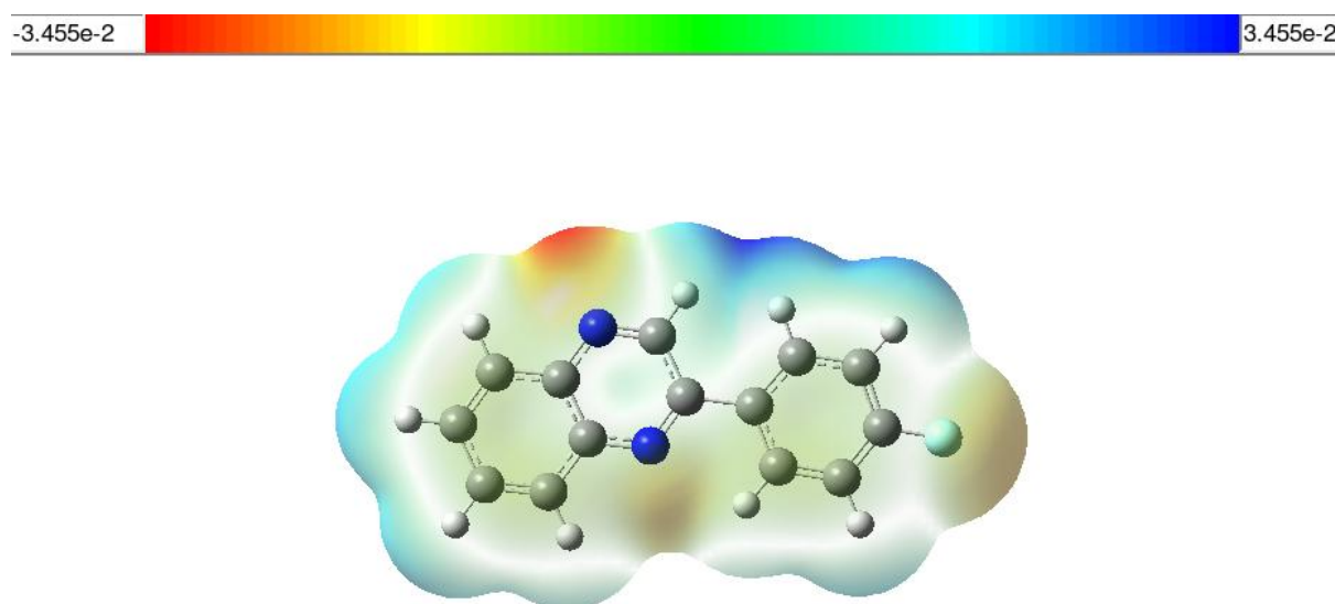
Figure 3. Molecular Electrostatic Potential Surface Map (MEP) of The 2-(4-fluorophenyl)quinoxaline
