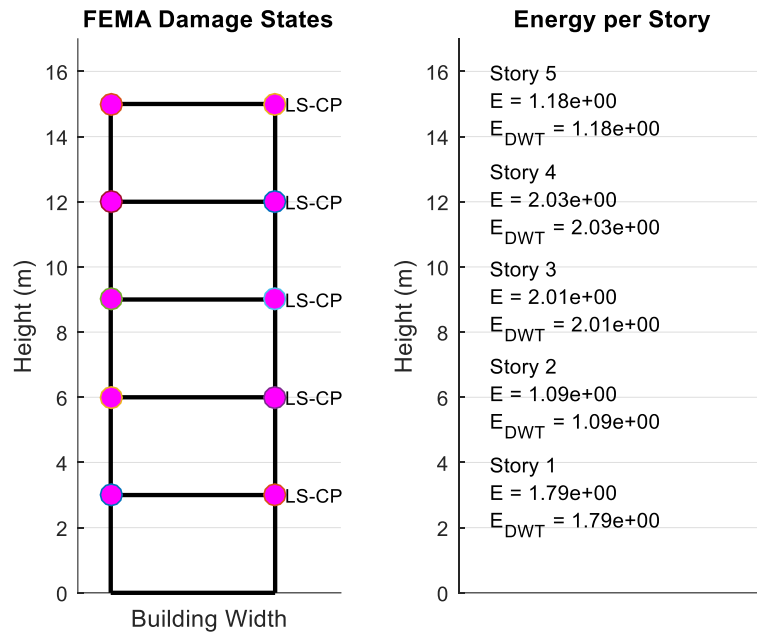
Figure 2. Damage states and corresponding energies under far-fault earthquakes
