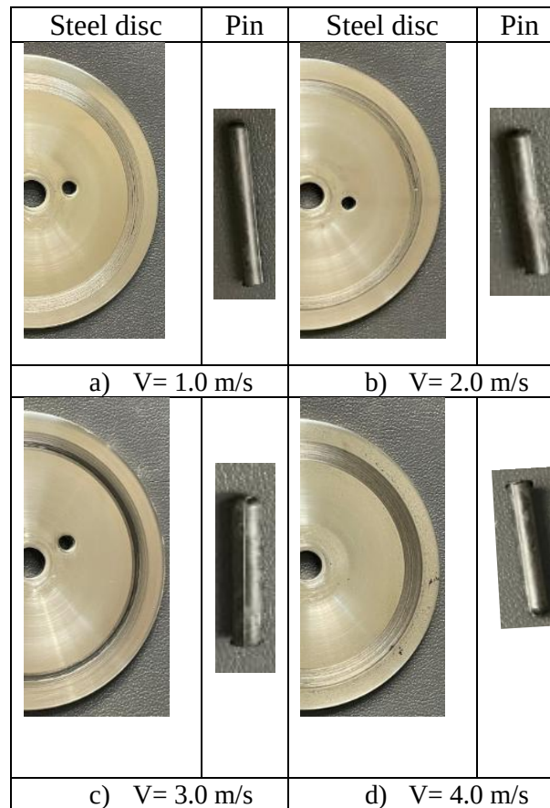
Figure 7. Camera images of the stainless steel wear surface in contact with PA66/30CF composite at different speeds: a) 1.0 m/s, b) 2.0 m/s, c) 3.0 m/s and d) 4.0 m/s
